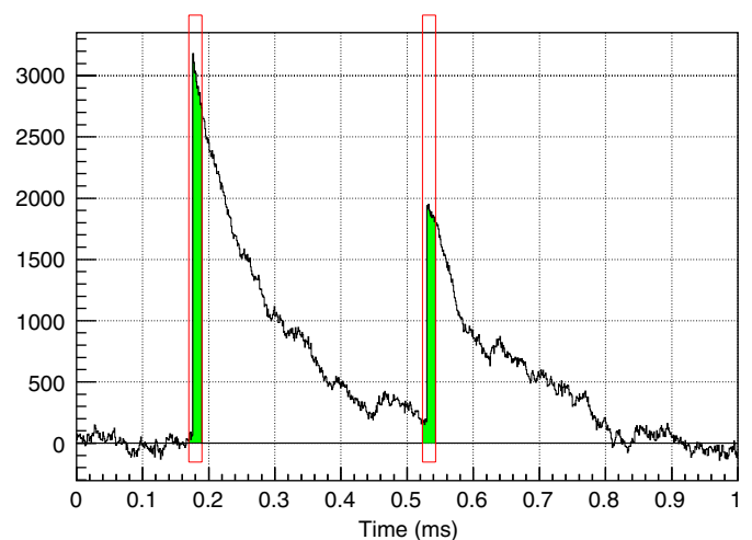
Fig. 1. Example of the output of a charge preamplifier over a long time scale. Two distinct events can easily be seen. The shaded areas correspond to the time windows available to an event-based system.
