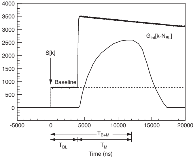
Fig. 3. Definition of the quantities used in the text. The signal S[k] has been acquired with a finite T_{BL} ( T_{BL} = 4 \mu\text{s} in the figure).
