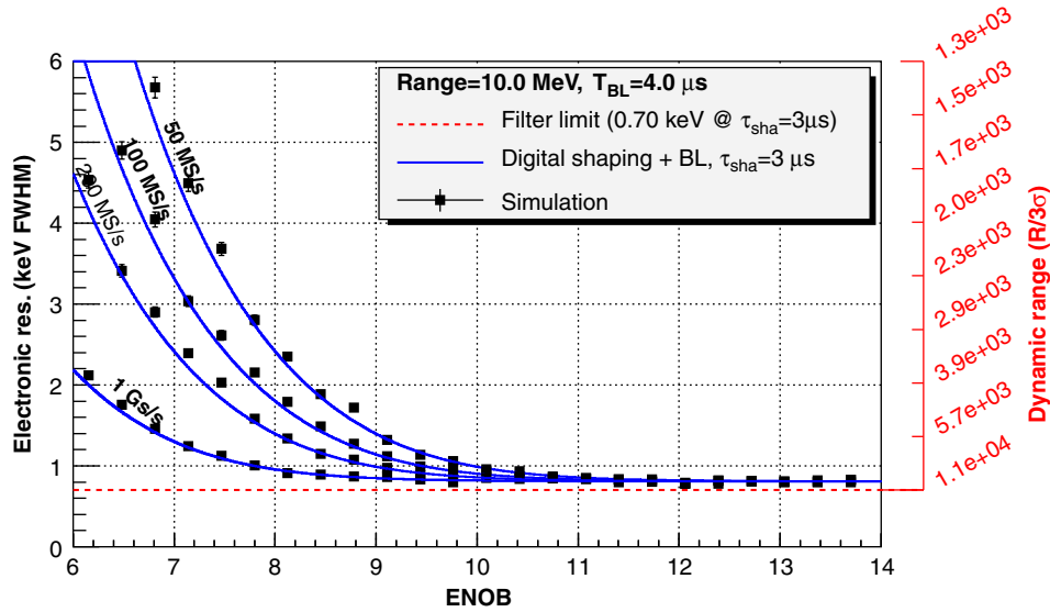
Fig. 6. Same as Fig. 5, but using a baseline time T_{BL} = 4 \mu\text{s} .
