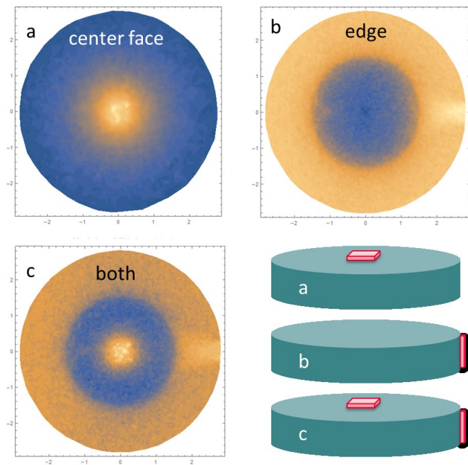
Fig. 3. Optical simulation results showing light collection probability maps for three example SiPM placement positions.
