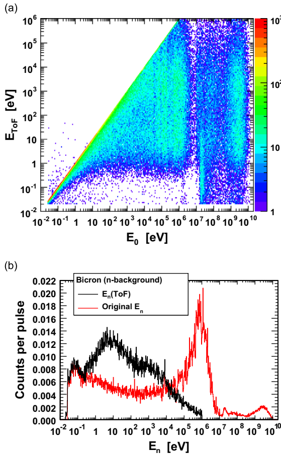
Fig. 8. Time structure of the neutron background simulated for a ^{nat}\text{C} sample in the Bicorn detector. Top panel (a): correlations between the primary neutron energies and those reconstructed from the time of flight. Bottom panel (b): projections of the top plot on both axes. Only the spectrum of reconstructed energies is experimentally accessible.
