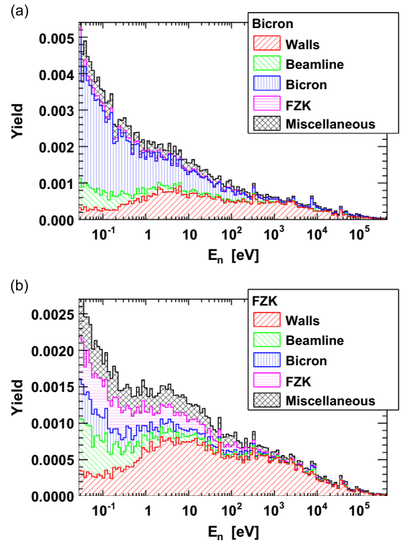
Fig. 10. Stacked contributions to the neutron background yield of ^{nat}\text{C} for both \text{C}_6\text{D}_6 detectors – Bicorn (a) and FZK (b) – coming from the different sets of experimental components. Note that absolute scales for two detectors differ by a factor of 2.
