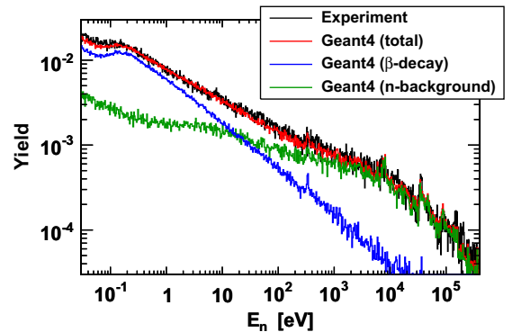
Fig. 7. Comparison between the experimental and simulated yield for the ^{nat}C sample 1 cm in thickness and 2 cm in diameter. The contribution of the true neutron background – caused by the scattering of the primary neutrons – is shown separately from the detection of \beta -rays emitted by the radioactive residuals produced by neutron inelastic reactions in the sample. (For interpretation of the references to color in this figure caption, the reader is referred to the web version of this article.)
