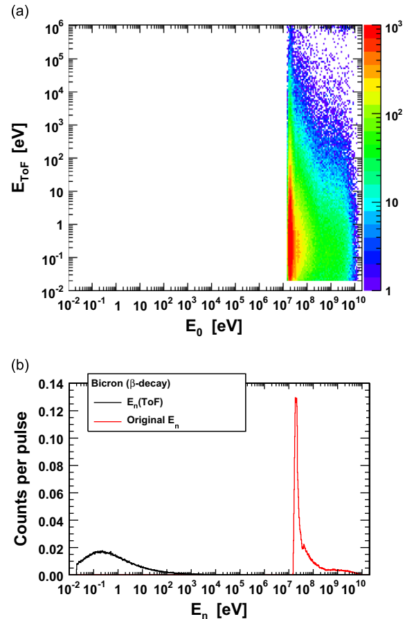
Fig. 9. Time structure of the detected \beta -rays from the decay of radioactive isotopes produced by the neutron inelastic reactions in ^{nat}\text{C} sample. The plots are analogous to those from Fig. 8. The spectrum of primary neutron energies from bottom panel (b) bears the signature of the cross-section for the dominant ^{12}\text{C}(n, p)^{12}\text{B} reaction.
