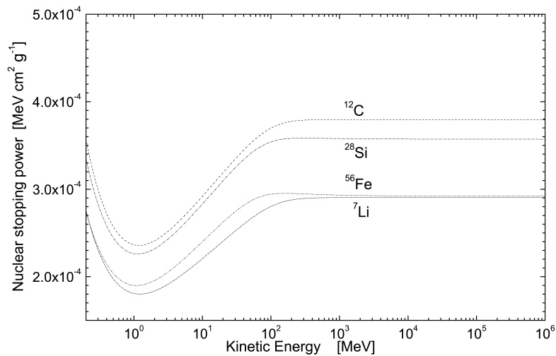
Fig. 8.5: In \text{MeVcm}^2/\text{g} , nuclear stopping powers in {}^7\text{Li} , {}^{12}\text{C} , {}^{28}\text{Si} and {}^{56}\text{Fe} calculated from Eq.(8.74) and divided by the density of the material as a function of the kinetic energy of electrons from 200 keV up to 1 TeV.
