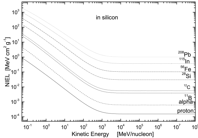
Fig. 8.3: Non-ionizing stopping power from Ref. [MJB11] calculated using Eq.(8.33) in silicon is shown as a function of the kinetic energy per nucleon, from 50 keV/nucleon up 100 TeV/nucleon, for protons, \alpha -particles and ^{11}\text{B} , ^{12}\text{C} , ^{28}\text{Si} , ^{56}\text{Fe} , ^{115}\text{In} , ^{208}\text{Pb} nuclei. The threshold energy for displacement is 21 eV in silicon.
