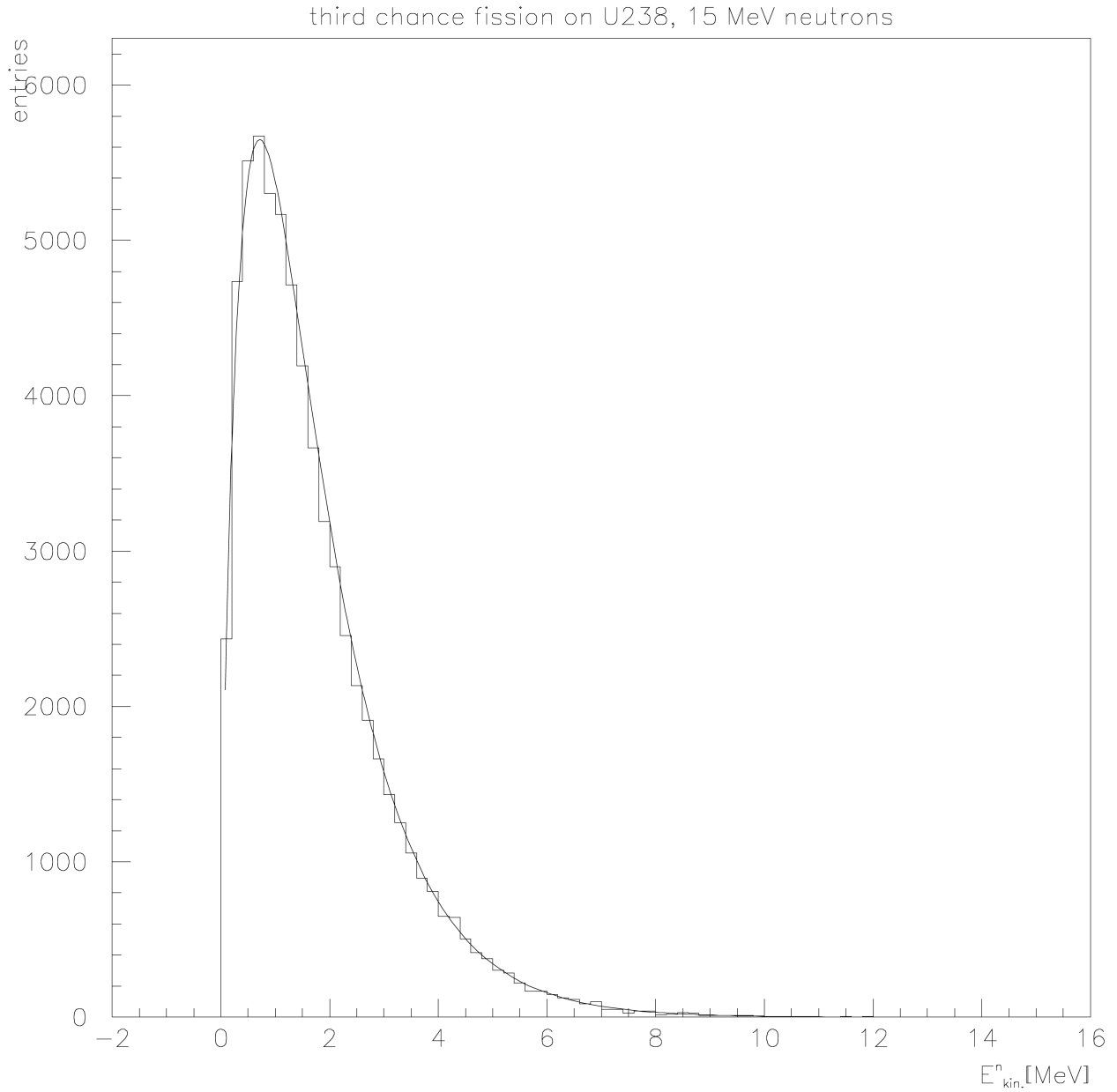
Fig. 39.3: Comparison of data and Monte Carlo for fission neutron energy distributions for induced fission by 15 MeV neutrons on uranium ( 238 U). The curve represents evaluated data and the histogram is the Monte Carlo prediction.
