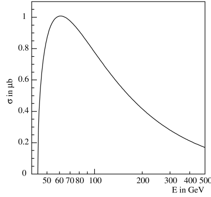
Fig. 10.6: Total cross section for the process e^+e^- \rightarrow \mu^+\mu^- as a function of the positron energy E in the laboratory system.
