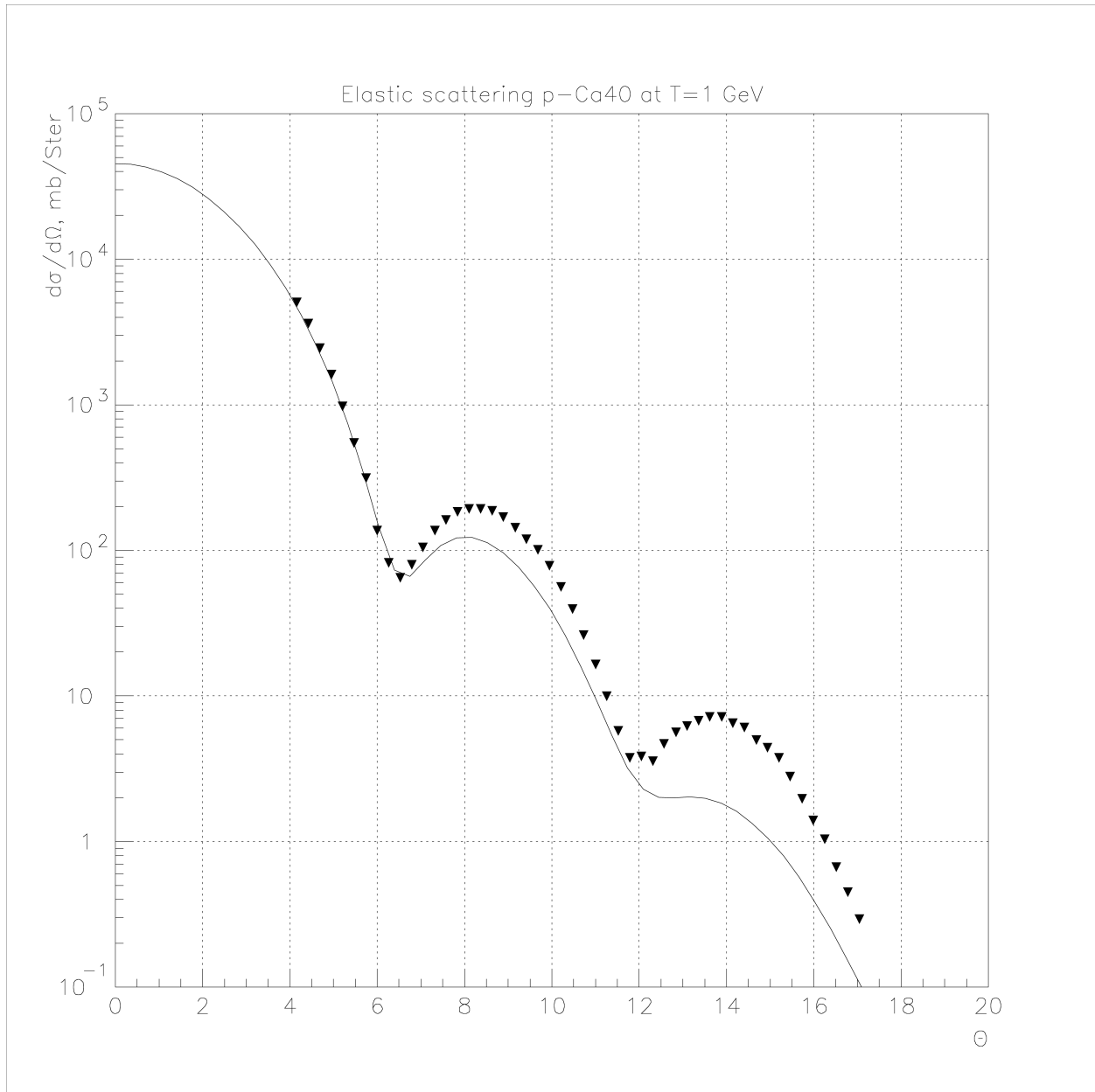
Fig. 23.6: Elastic proton scattering on 40 Ca at 1 GeV.
