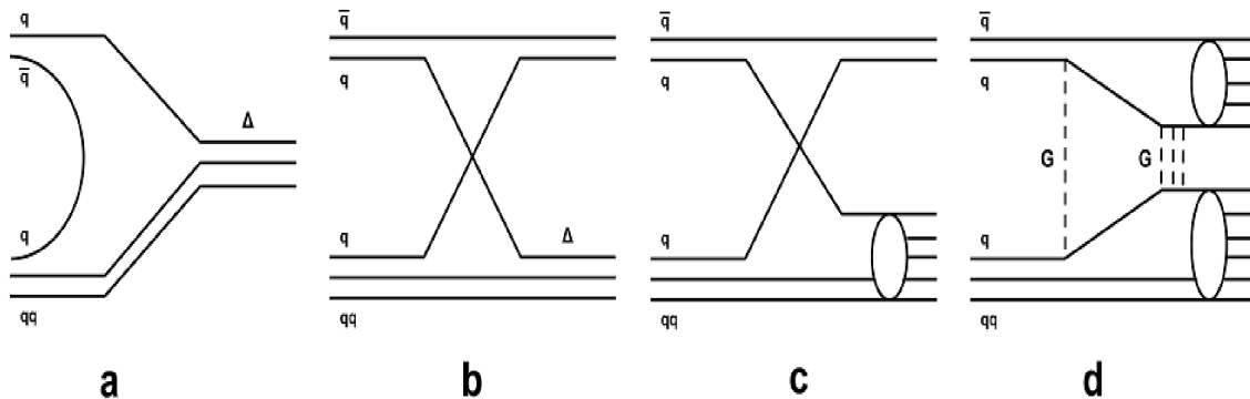
Fig. 3.14: Quark flow diagrams of \pi N interactions.
