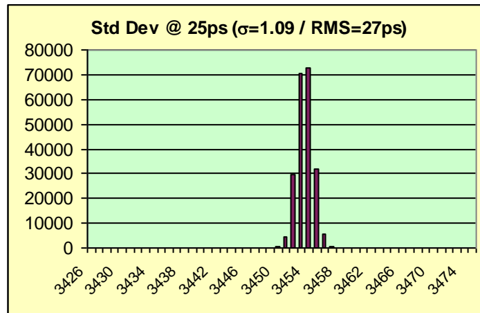
Fig. 2.13 RMS example after INL compensation
